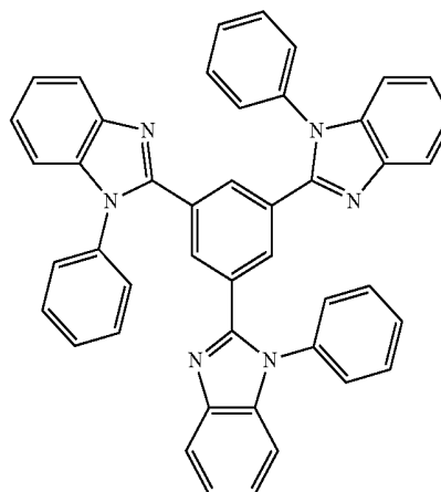
Chemical Formula 7
