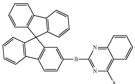
Chemical Formula 4
