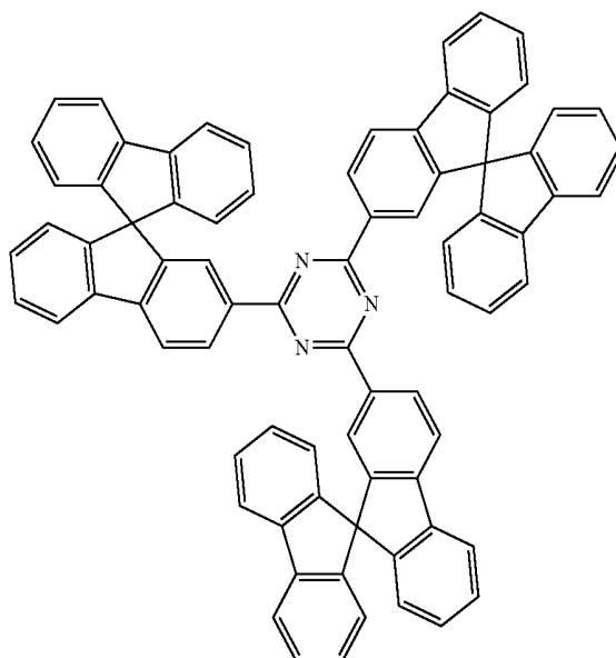
Chemical Formula 1-2
