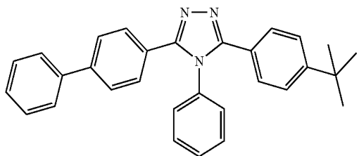
Chemical Formula 8
