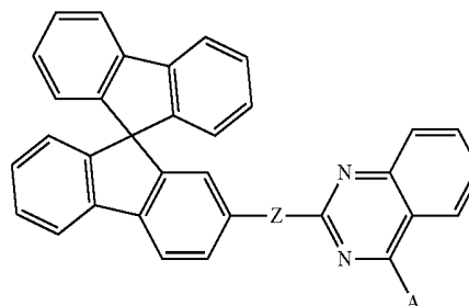
Chemical Formula 3
