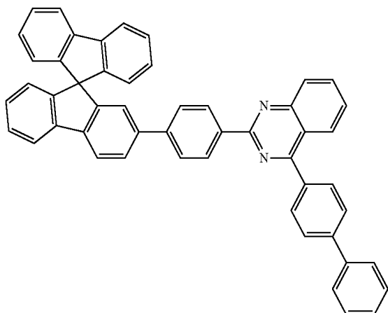
Chemical Formula 4-2
