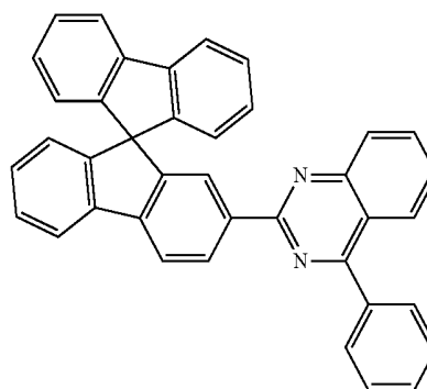
Chemical Formula 3-1
