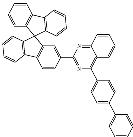
Chemical Formula 3-2
