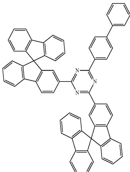
Chemical Formula 1-3
