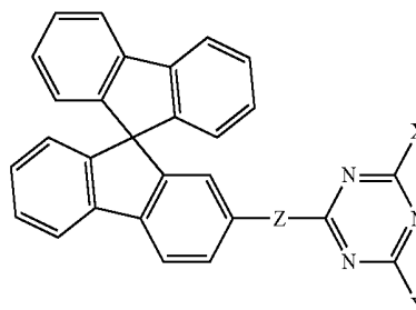
Chemical Formula 2
