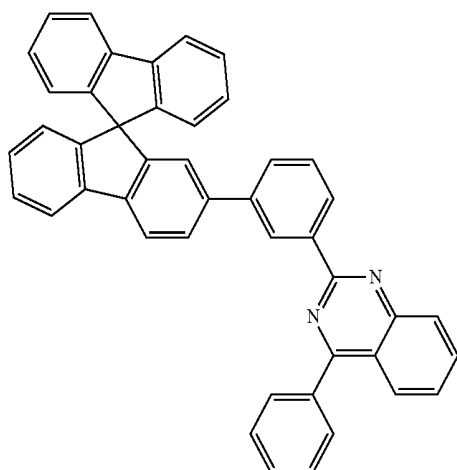
Chemical Formula 4-1
