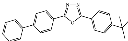
Chemical Formula 8
