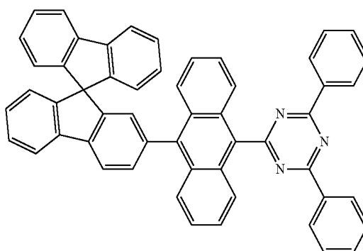
Chemical Formula 2-4
