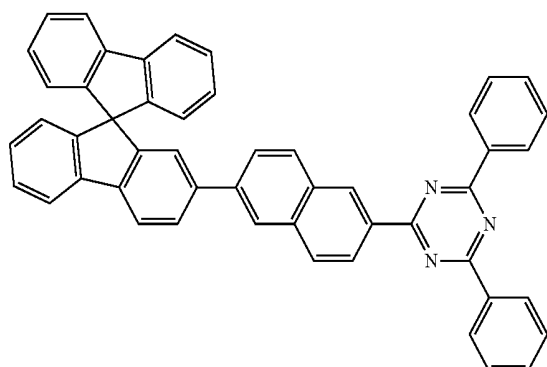
Chemical Formula 2-2
