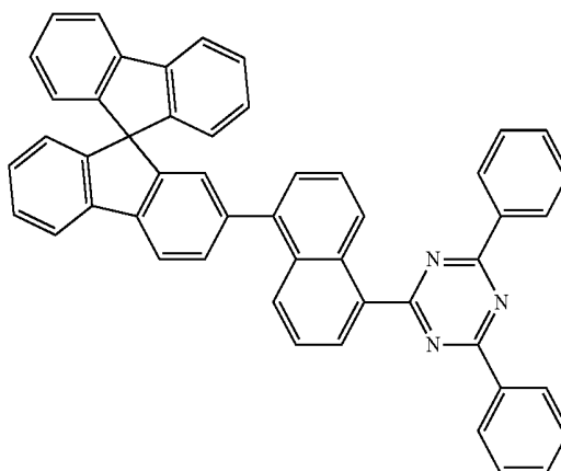
Chemical Formula 2-3
