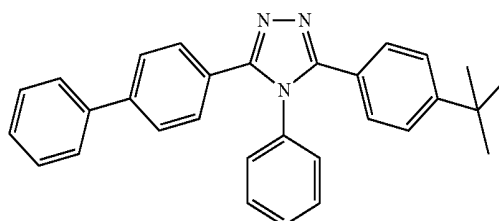
Chemical Formula 8
