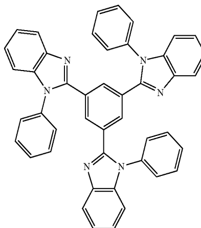
Chemical Formula 7
