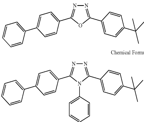
Chemical Formula 7
