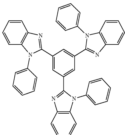
Chemical Formula 7
