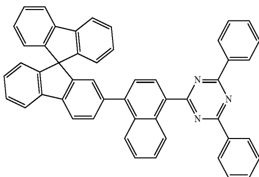
Chemical Formula 2-1
