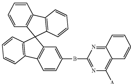
Chemical Formula 4
