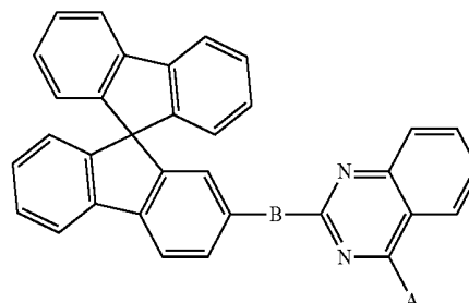
Chemical Formula 4
