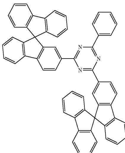
Chemical Formula 1-2
