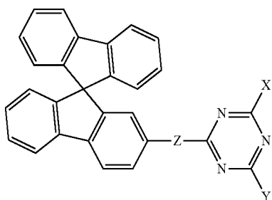
Chemical Formula 2
