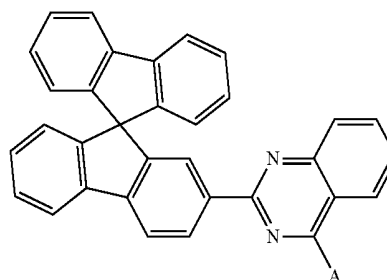
Chemical Formula 3
