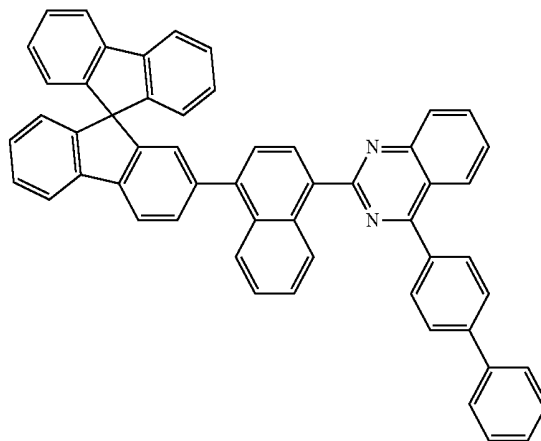
Chemical Formula 4-4
