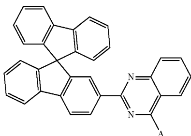
Chemical Formula 3
